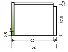
BASI H 78 BASE UNITS H 78
